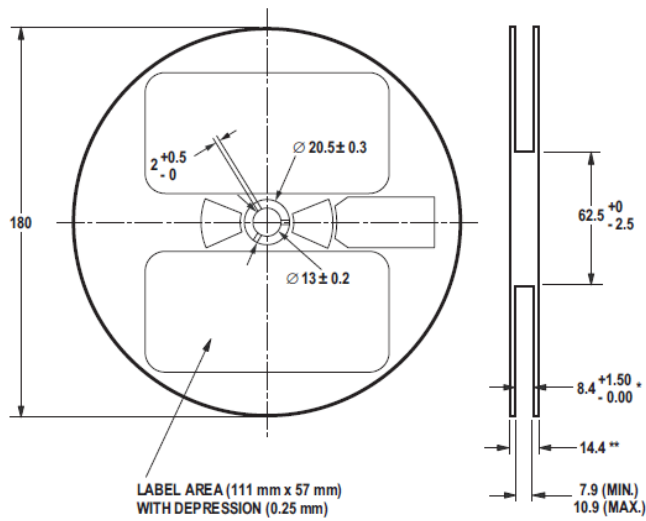
Figure 11. Reel dimensions
